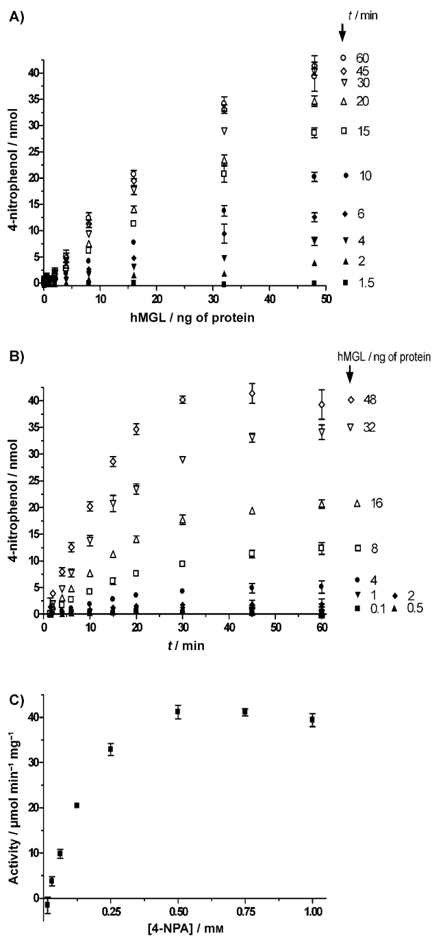
Figure 2. 4-NPA hydrolysis by human MGL. 4-NPA hydrolysis by MGL is A) protein concentration dependent, and B) time dependent. C) Varying the substrate concentration leads to a Michaelis–Menten-type curve ( K_m = 0.20 \pm 0.03 mM and V_{\max} = 52.2 \pm 2.3 \mu\text{mol min}^{-1} \text{mg}^{-1} ).
